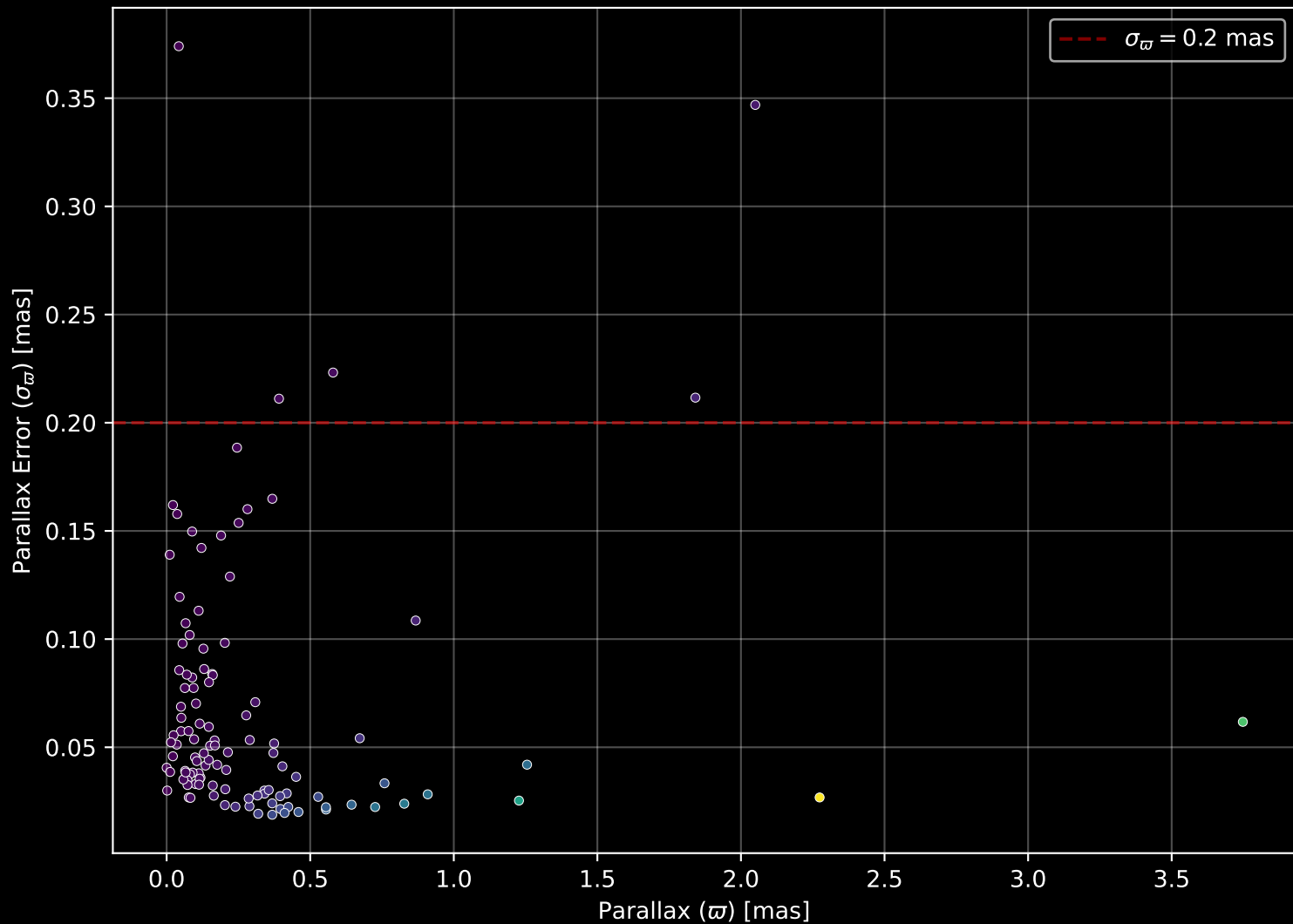
APOGEE DR17 Field: [004-02] Parallax Quality (n= 113)
