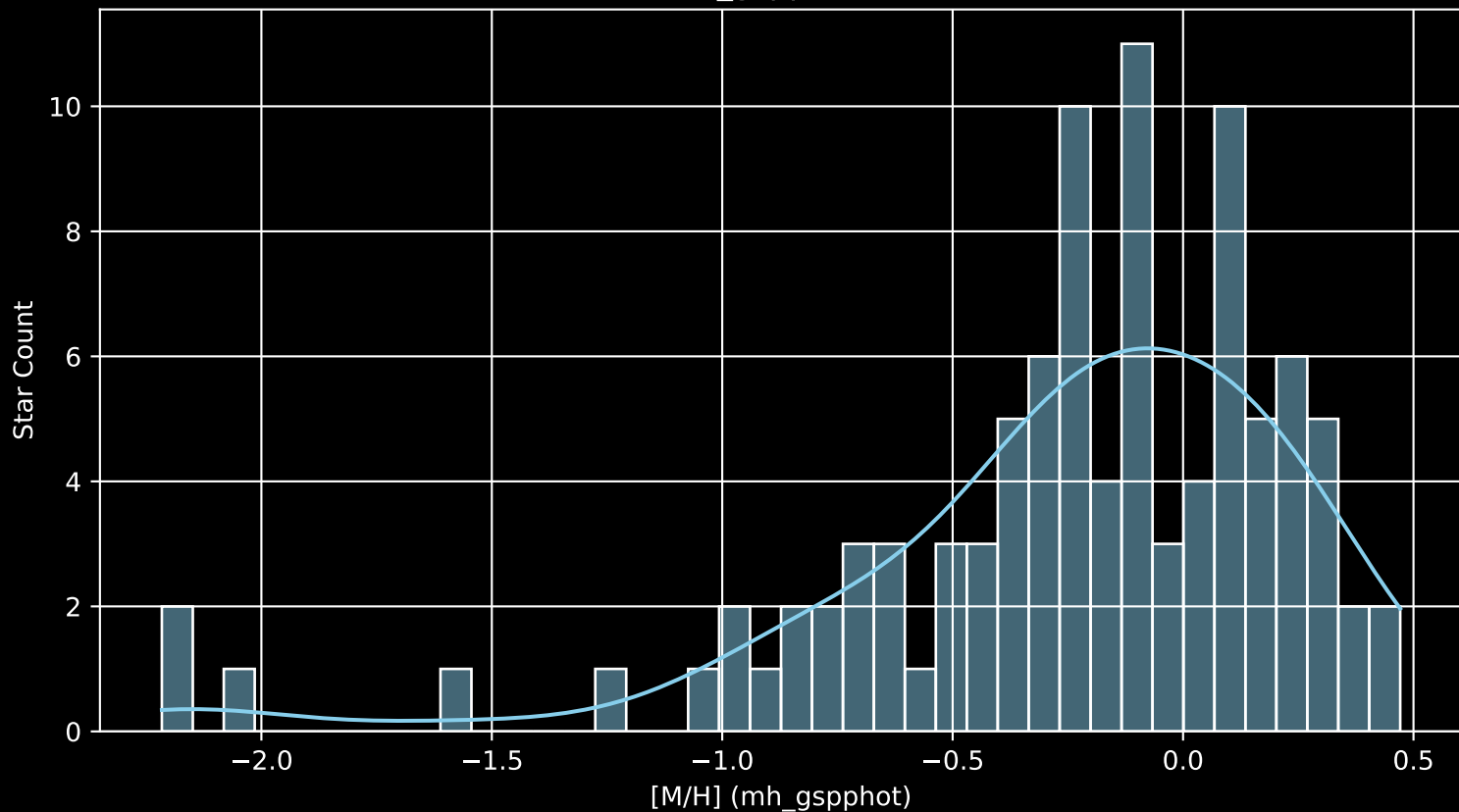
APOGEE DR17 Field: [004-02 [M/H] (mh_gspphot) (n= 99)
