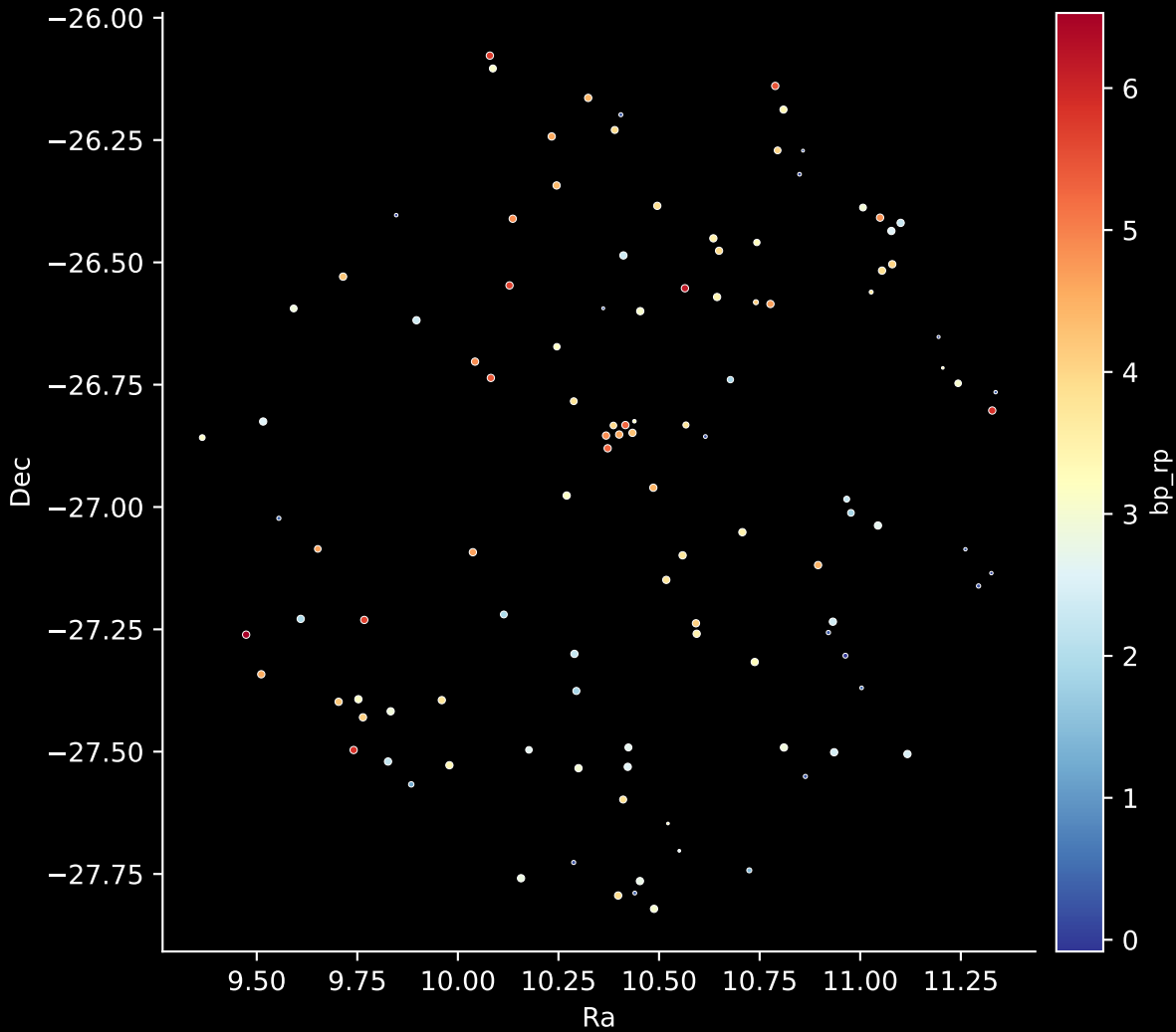
APOGEE DR17 Field: [004-02] Stars: 113
