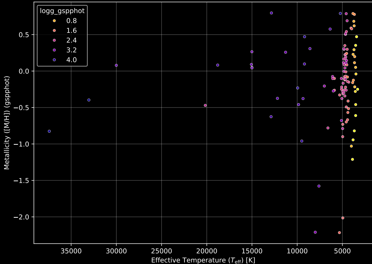
APOGEE DR17 Field: [004-02] Stellar Population Parameters (n= 113)
