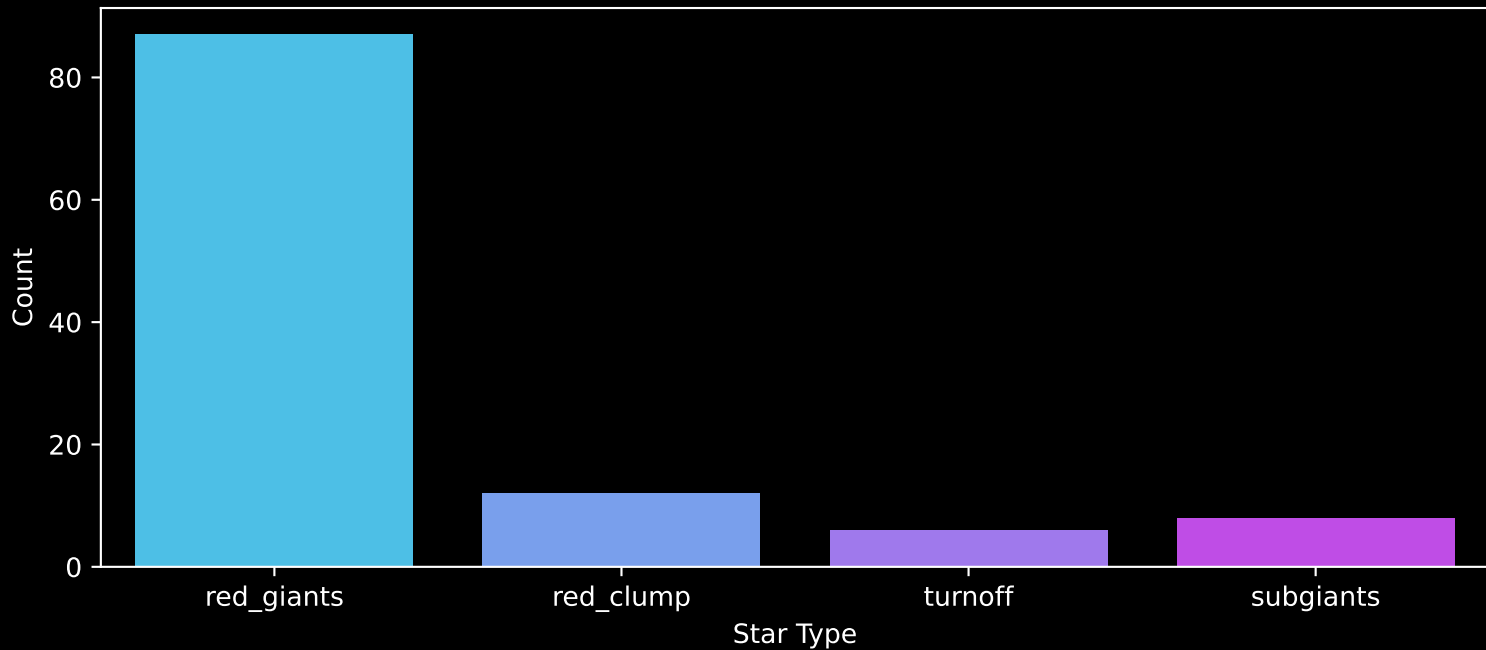
APOGEE DR17 Field: [004-02] Count plot of Star Type
