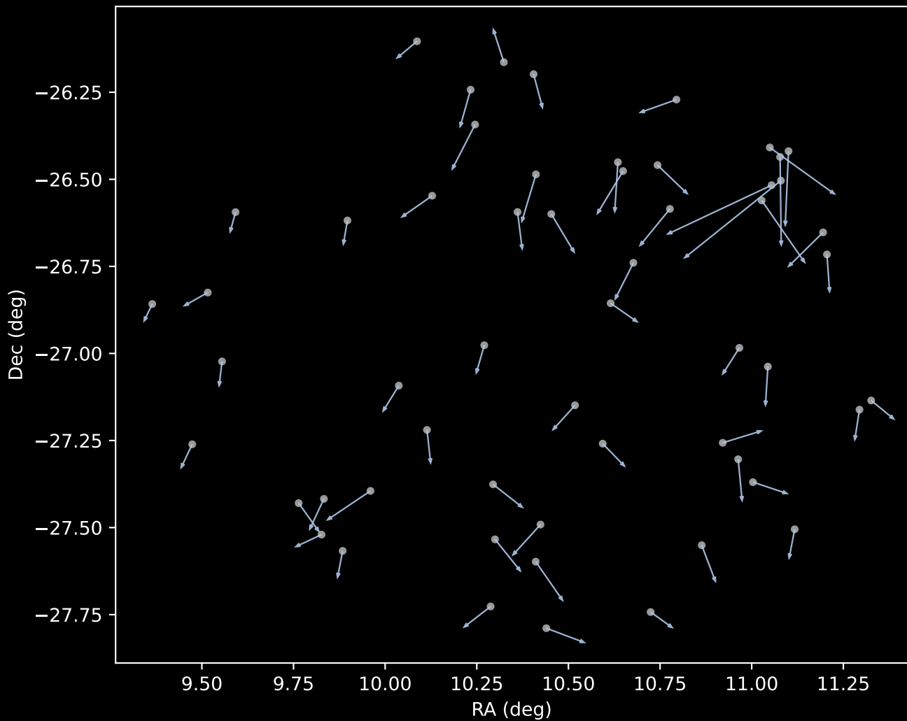
APOGEE DR17 Cluster 1 Proper Motion Vectors (n=56)
