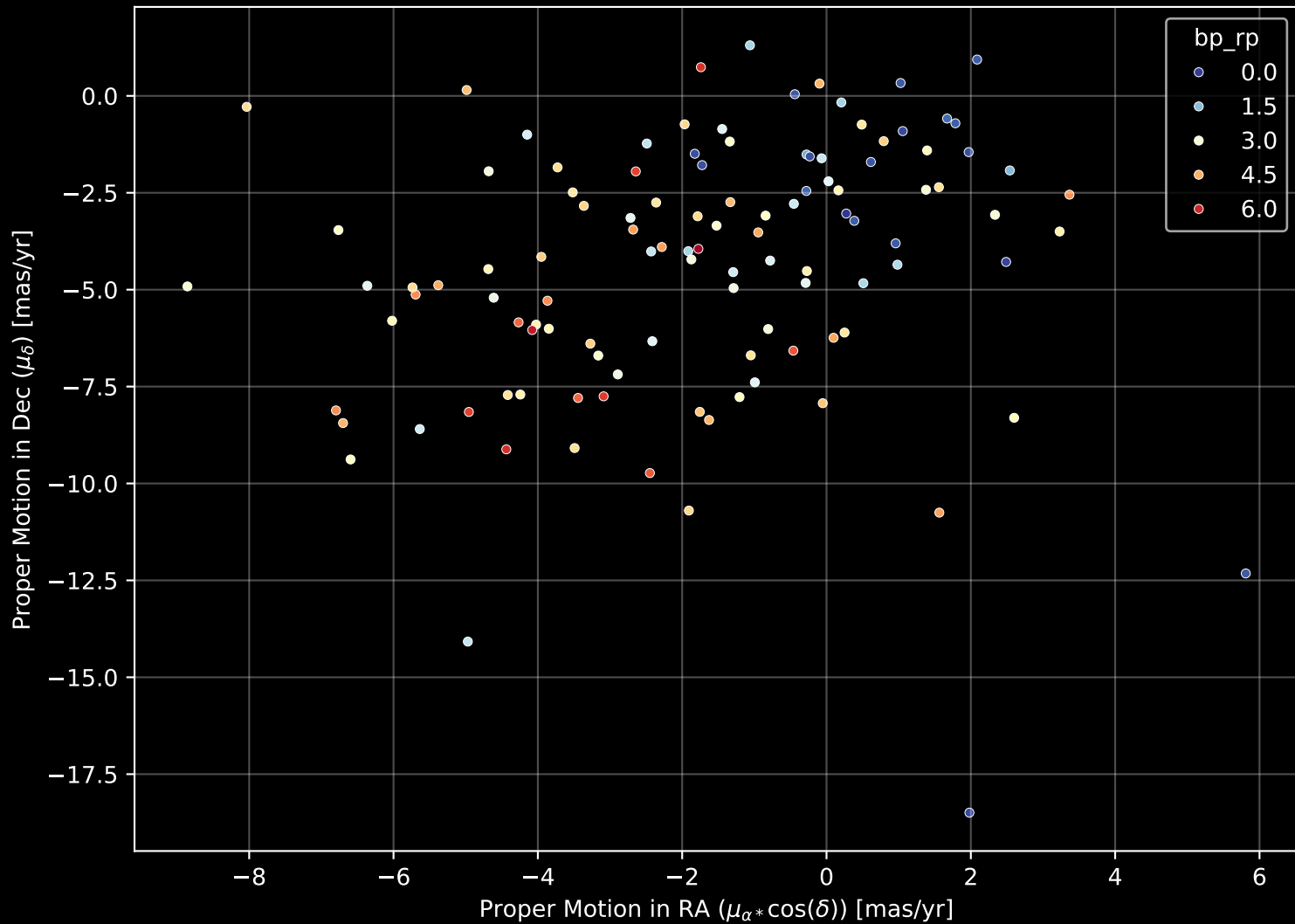
APOGEE DR17 Field: [004-02] Proper Motion Diagram (n= 113)
