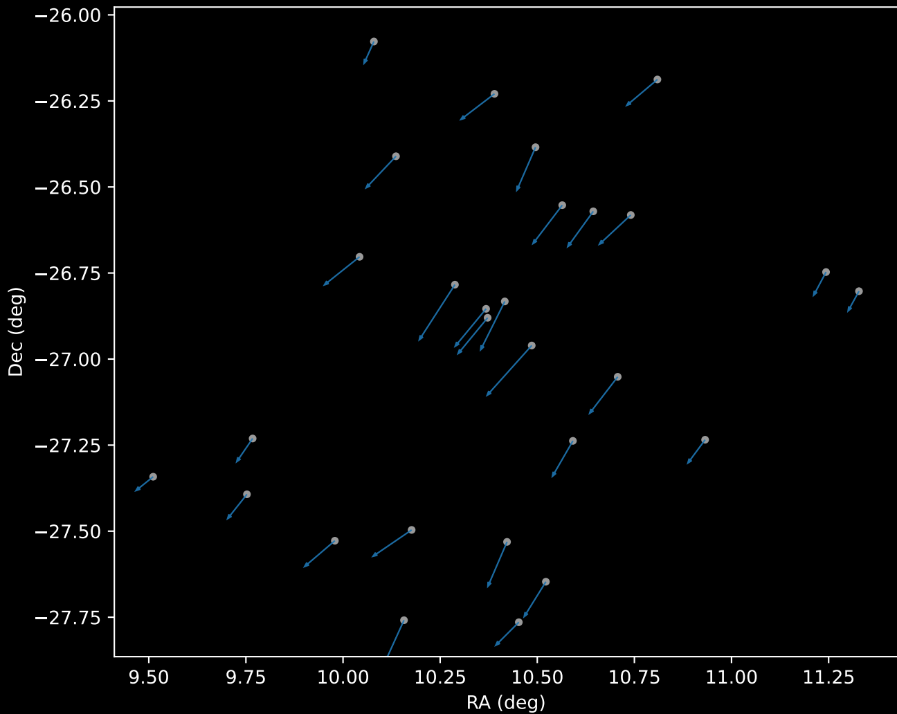
APOGEE DR17 Cluster 0 Proper Motion Vectors (n=28)
