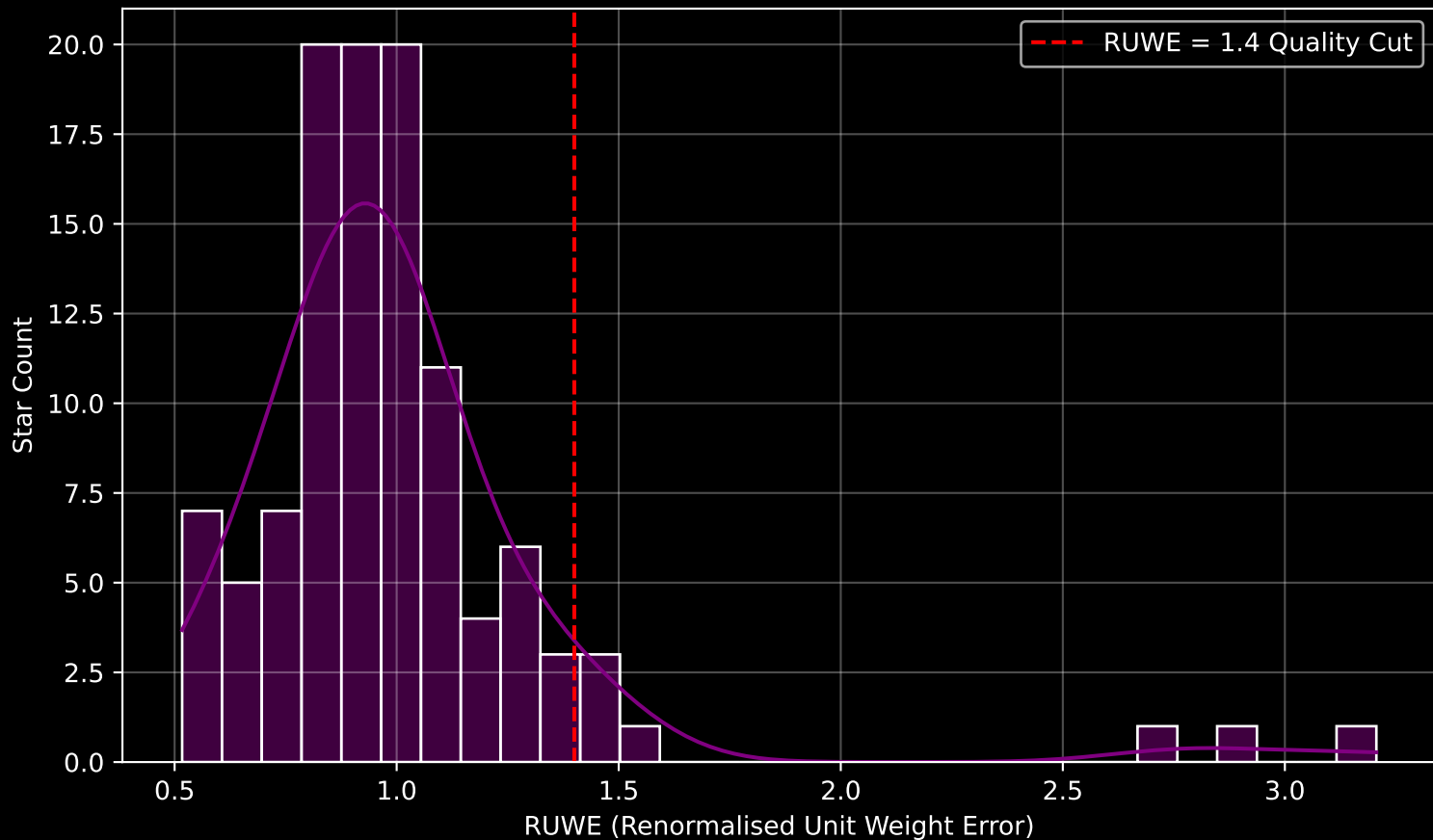
GAPOGEE DR17 Field [004-02] RUWE Distribution (n= 110)
